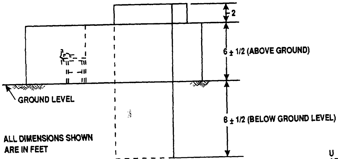
Figure 5-8. Pitch-in barricade.
